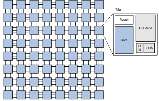
Figure 5: Configuration of a baseline 64-core multi-processor.
