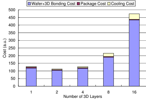
Figure 6: Cost break-down of a 32-core processor with homogeneous partitioning strategy.
