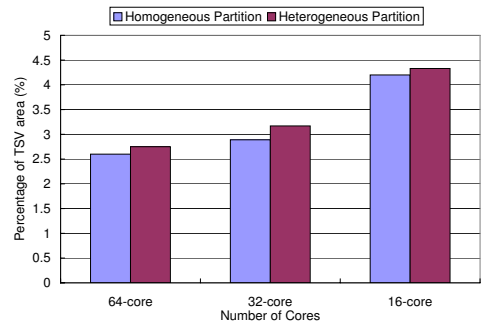
Figure 10: Compare the TSV area of 16-, 32- and 64-core multiprocessors using homogeneous and heterogeneous partitioning strategies.
