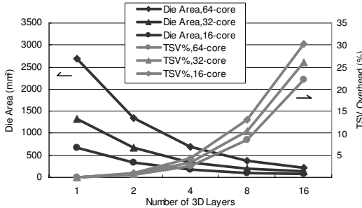
Figure 7: Analyzing the impact of TSV area overhead with homogeneous partitioning strategy.
