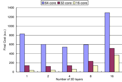
Figure 8: Final cost of 16-, 32- and 64-core multiprocessors with homogeneous partitioning strategy.
