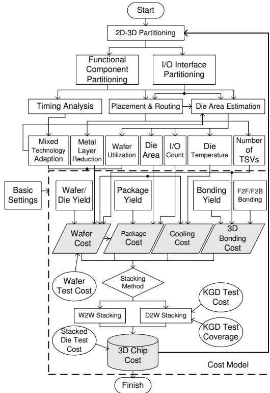
Figure 4: Integrating the proposed cost model with 3D EDA flow for cost-aware 3D many-core multi-processor design.
