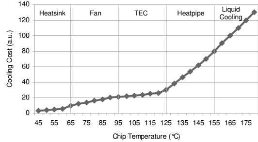
Figure 3: A plot for the proposed cooling cost model.
