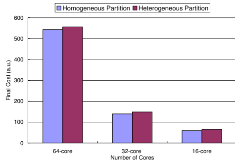
Figure 11: Compare the final costs of 16-, 32- and 64-core processors using homogeneous and heterogeneous partitioning strategies. All are partitioned into 4 3D layers.
