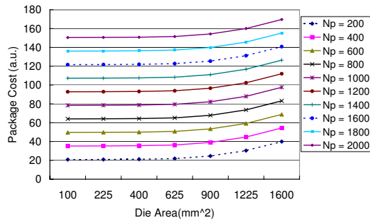
Figure 2: The package cost depends on both pin count and die area.
