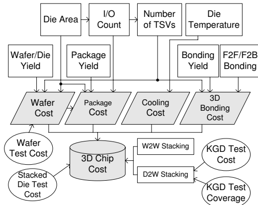
Figure 1: Overview of the proposed 3D many-core processor cost model.
