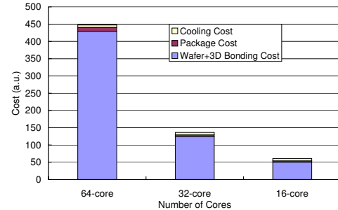
Figure 9: Cost break-down of 16-, 32- and 64-core multiprocessors with 4-layer heterogeneous partitioning strategy.
