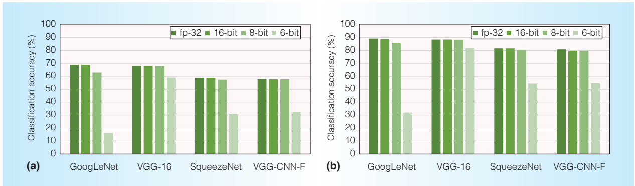
Figure 3. Quantization results for different CNN models. (a) Top-1 classification accuracy. (b) Top-5 classification accuracy.
