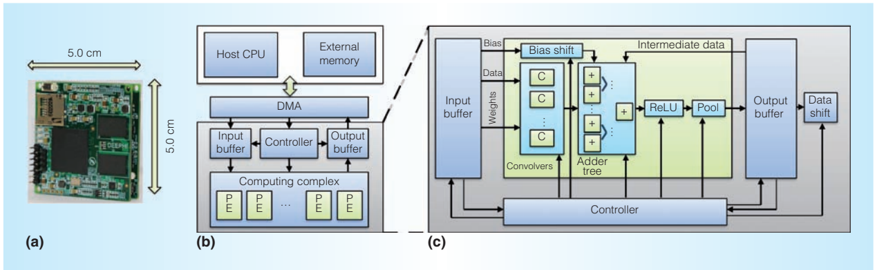
Figure 2. Aristotle architecture for the convolutional neural network (CNN) accelerator. (a) System board. (b) Overall system architecture. (c) Processing element (PE) architecture.
